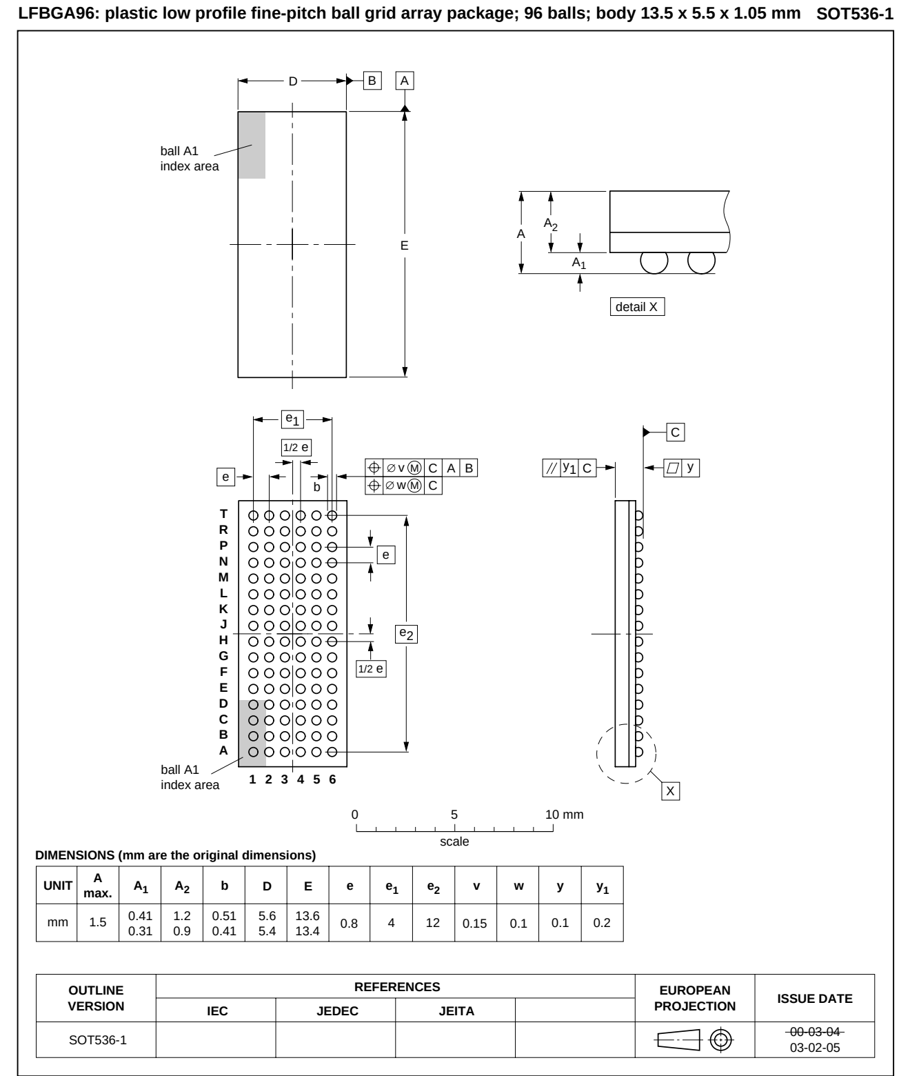
Fig 7. Package outline SOT536-1 (LFBGA96)
